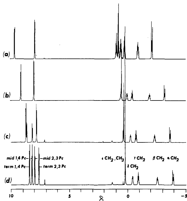
Figure 1. NMR spectra, 200 MHz: (a) (n\text{-C}_6\text{H}_{13})_3\text{SiOSiPcOSi}(n\text{-C}_6\text{H}_{13})_3 ; (b) (n\text{-C}_6\text{H}_{13})_3\text{SiO}(\text{SiPcO})_2\text{Si}(n\text{-C}_6\text{H}_{13})_3 ; (c) (n\text{-C}_6\text{H}_{13})_3\text{SiO}(\text{SiPcO})_3\text{Si}(n\text{-C}_6\text{H}_{13})_3 ; (d) (n\text{-C}_6\text{H}_{13})_3\text{SiO}(\text{SiPcO})_4\text{Si}(n\text{-C}_6\text{H}_{13})_3 .
